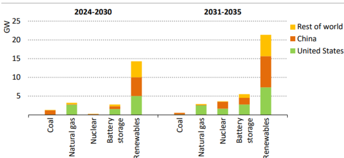
Chart 5: Annual Average Data Centre Power Capacity Additions by Fuel and Region: Base Case Outlook for 2024–2030 and 2031–2035
